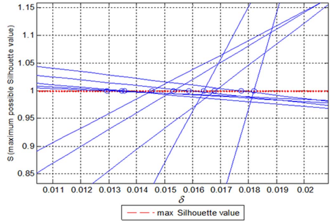
Fig. 6. Computation of interpolation nodes \eta using “fzero” simulation on the Lagrange's function S_I = (const.)_I.f(\delta_I) for the sample image in Table I.
