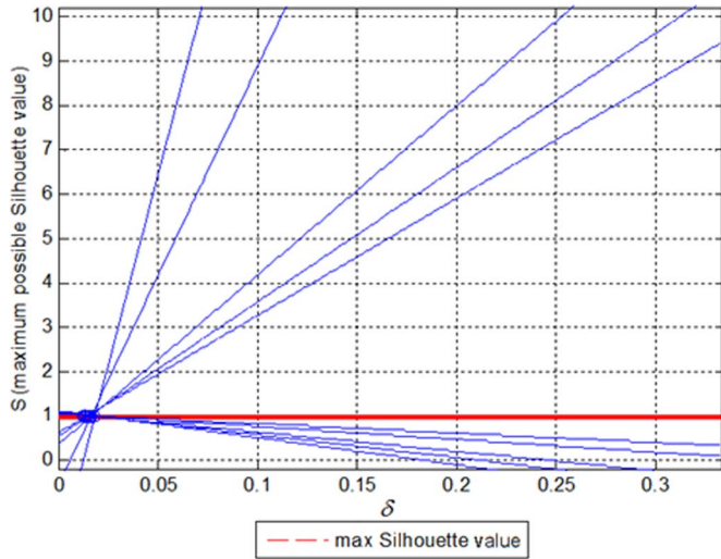
Fig. 5. Variation of S with threshold value \delta over the range [0, 0.3333] in the Lagrange's function S_I = (const.)_I.f(\delta_I) for the sample image in Table I.
