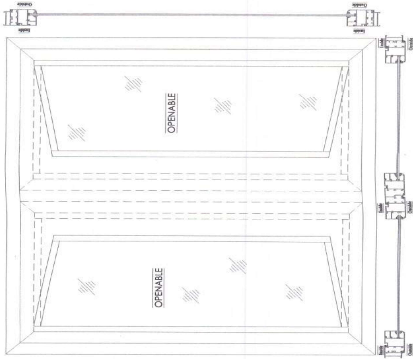
50mm Double window with center Flying Mullion
