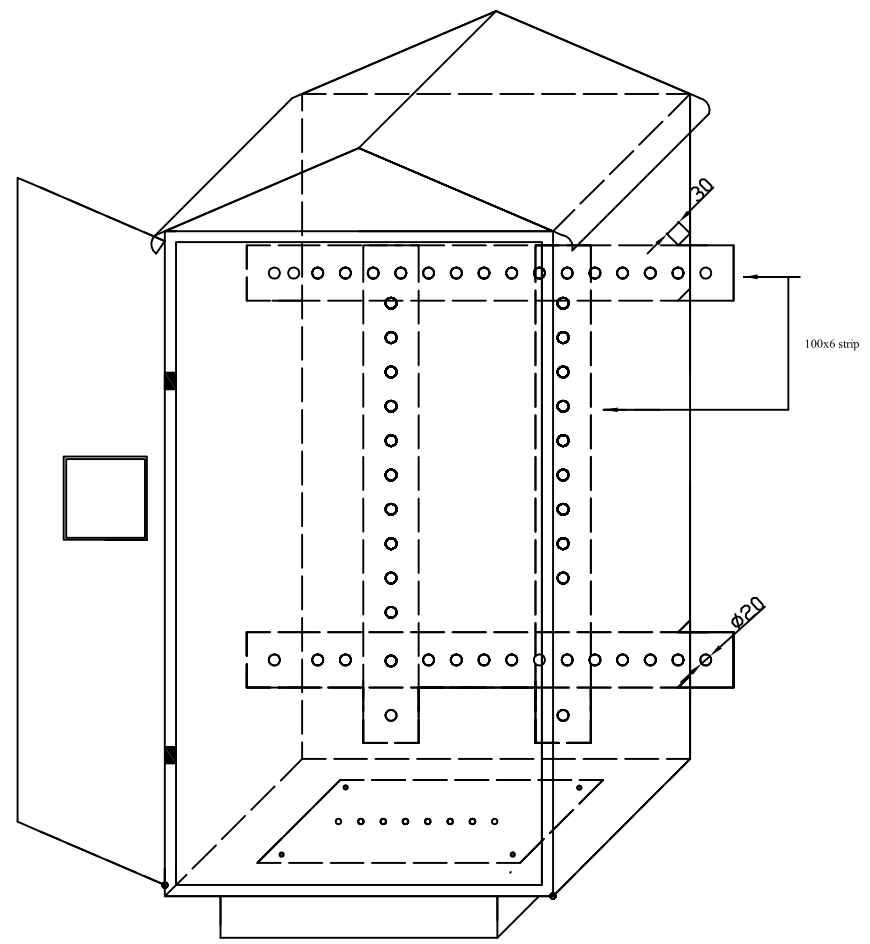
Isometric view of open box
