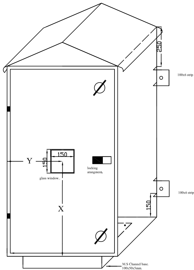
Isometric view of closed box.
