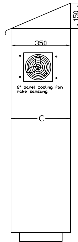
L.H.S view
